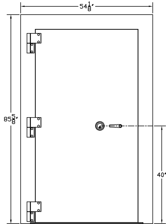
EXTERIOR ELEVATION
